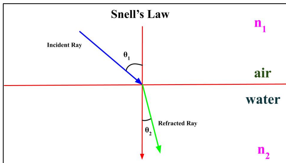
Figure 2: Snell's Law
